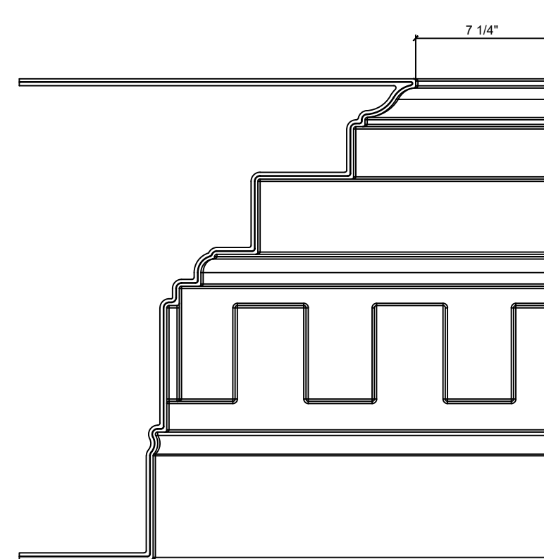
4 CR144x8 Elevation of Inside Corner SCALE 1:1
