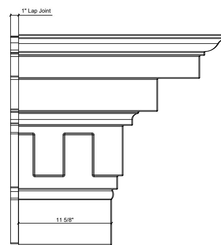
6 CR144x8 Elevation of Outside Corner SCALE 1:1
