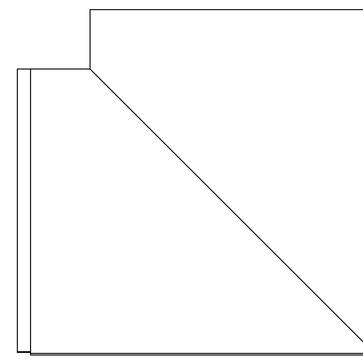
3 CR144x8 Outside Corner Top View SCALE 1:1
