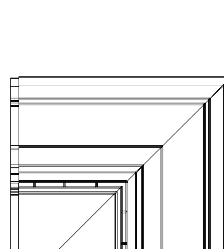
10 CR144x8 Outside Corner Under Side SCALE 1:1
