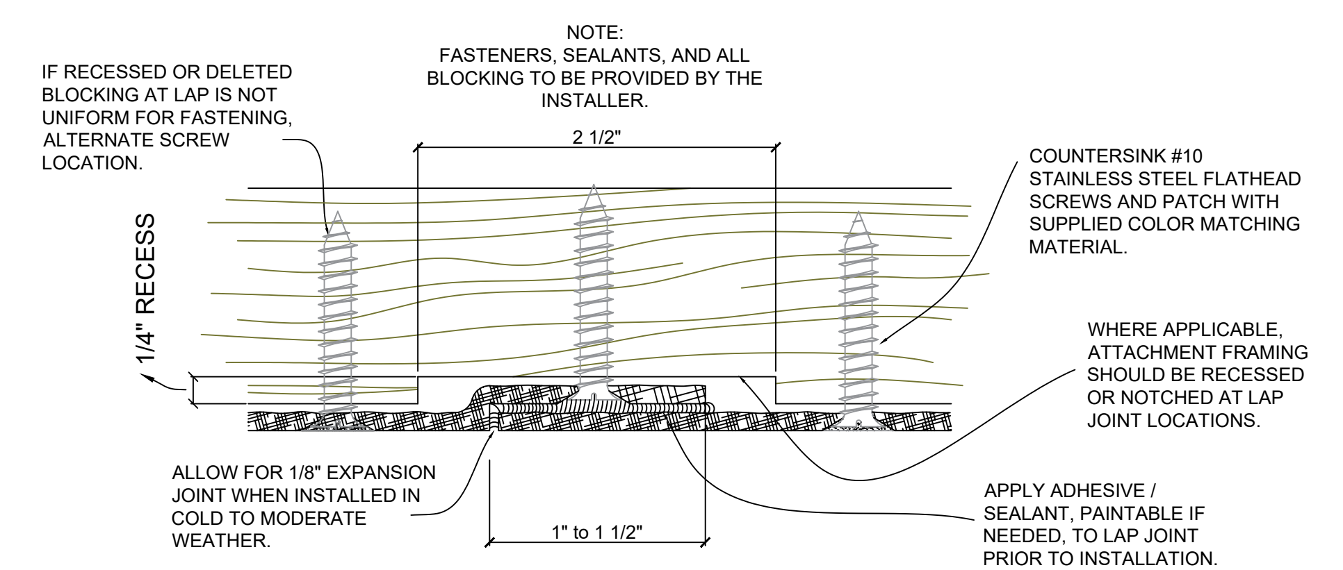
11 Typical Lap Joint Detail Not to Scale
