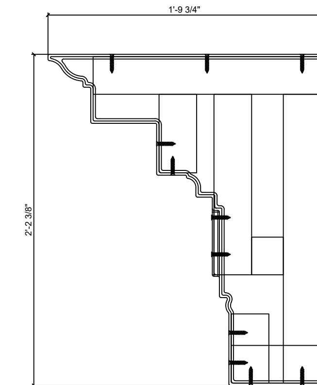
7 CR144x8 Cross Section SCALE 1:1
