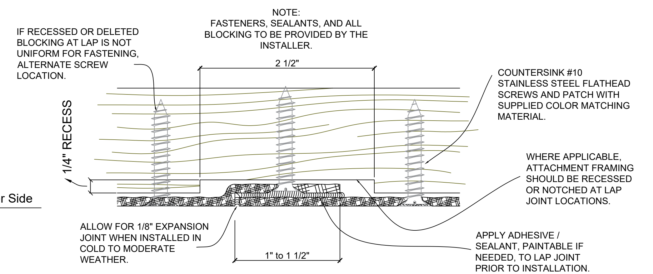
11 Typical Lap Joint Detail Not to Scale
