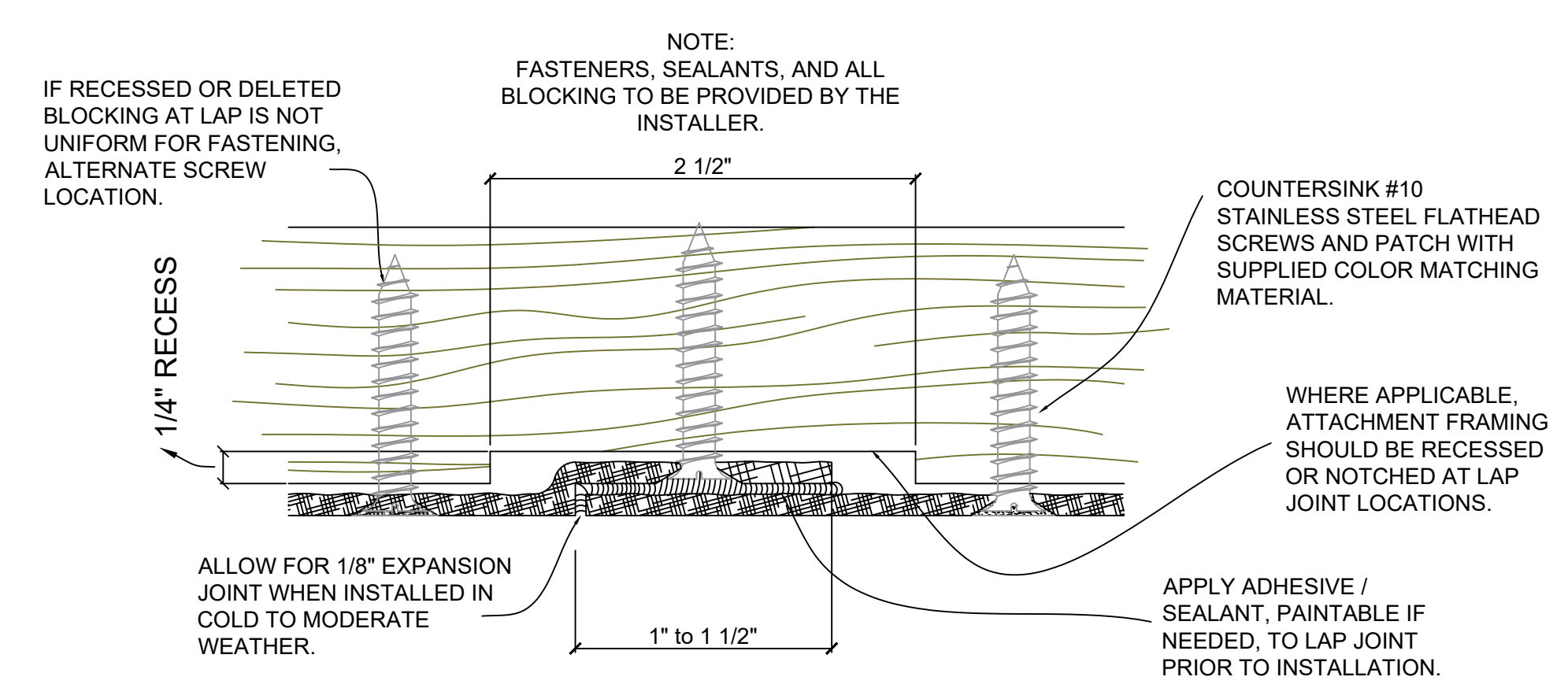
11 Typical Lap Joint Detail Not to Scale
