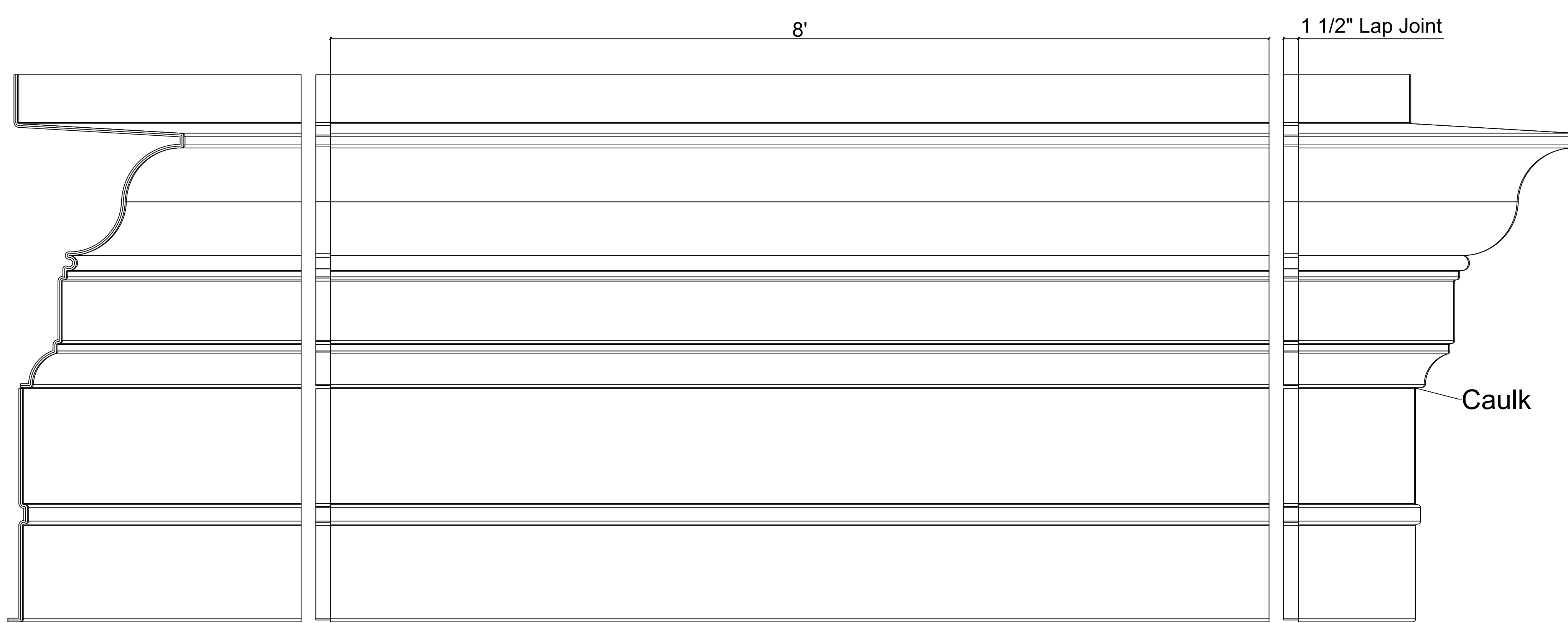
4 CR165x8 Elevation of Inside Corner SCALE 1:1
