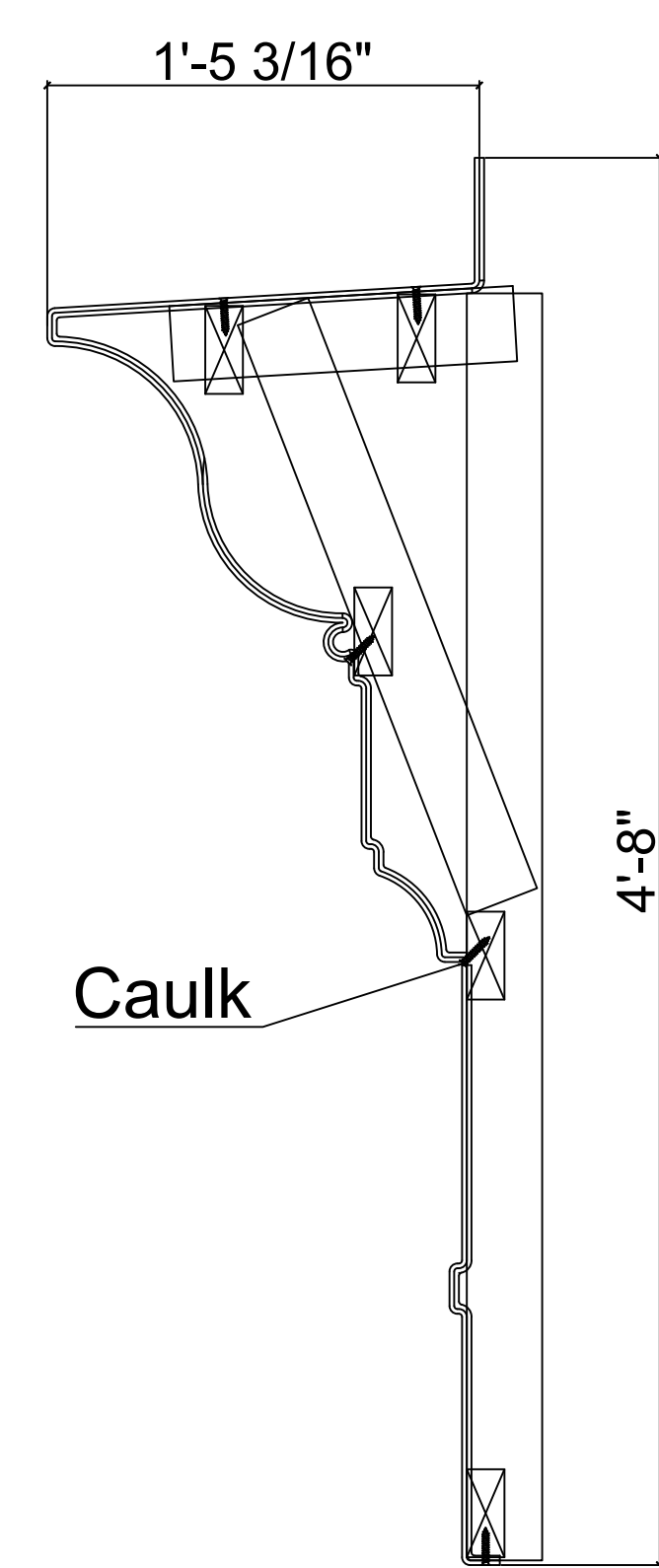
7 CR165x8 Cross Section SCALE 1:1
