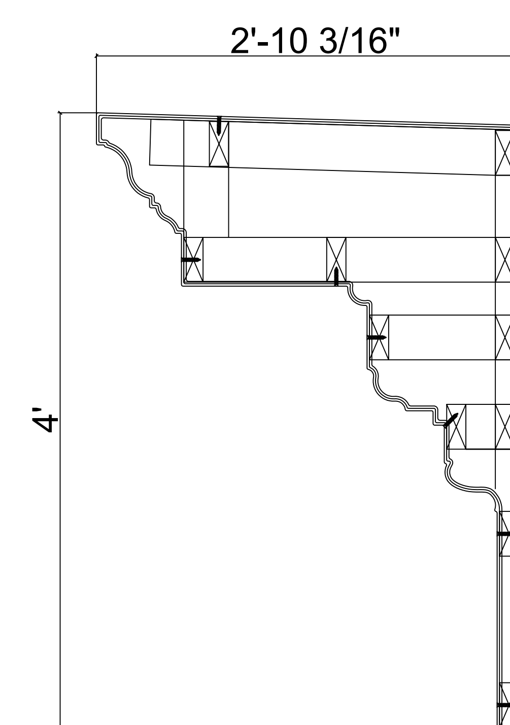
7 CR170x6 Cross Section SCALE 1:1
