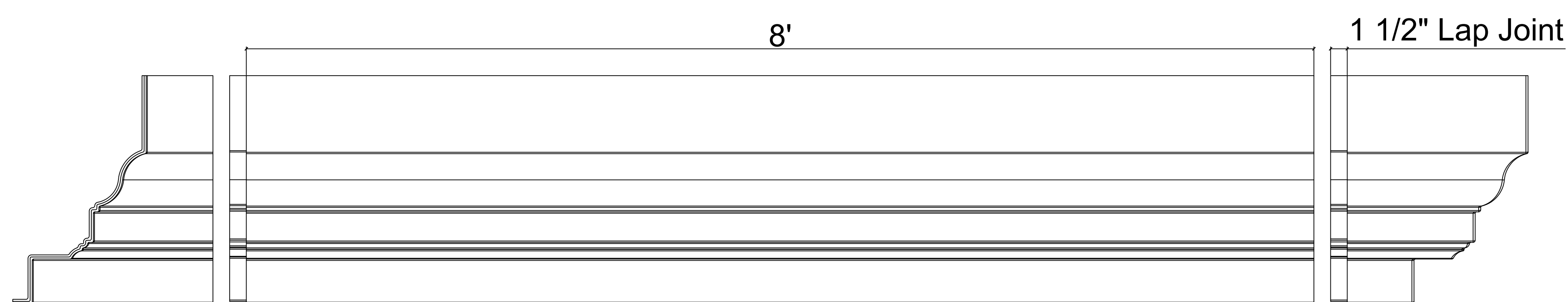
4 CR172x8 Elevation of Inside Corner SCALE 1:1
